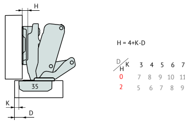
dobradiça 110° C35 recta 01.06.516 R
