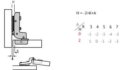
dobradiça 180° C35 curva-total 01.06.511 C
