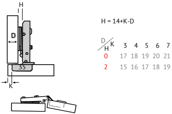
dobradiça 180° C35 reta 01.06.511 R
