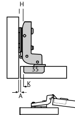
dobradiça mola C35 curva total Clip 01.06.515 C
