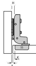
dobradiça mola C40 curva total 01.06.514 C
